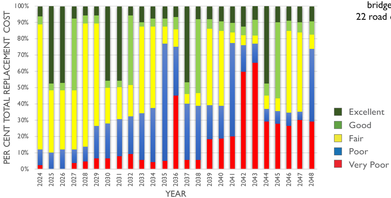
Projected annual performance of bridge assets
