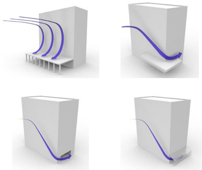
Image 2: Examples of Architectural details for Wind Control, Provided by RWDI.
