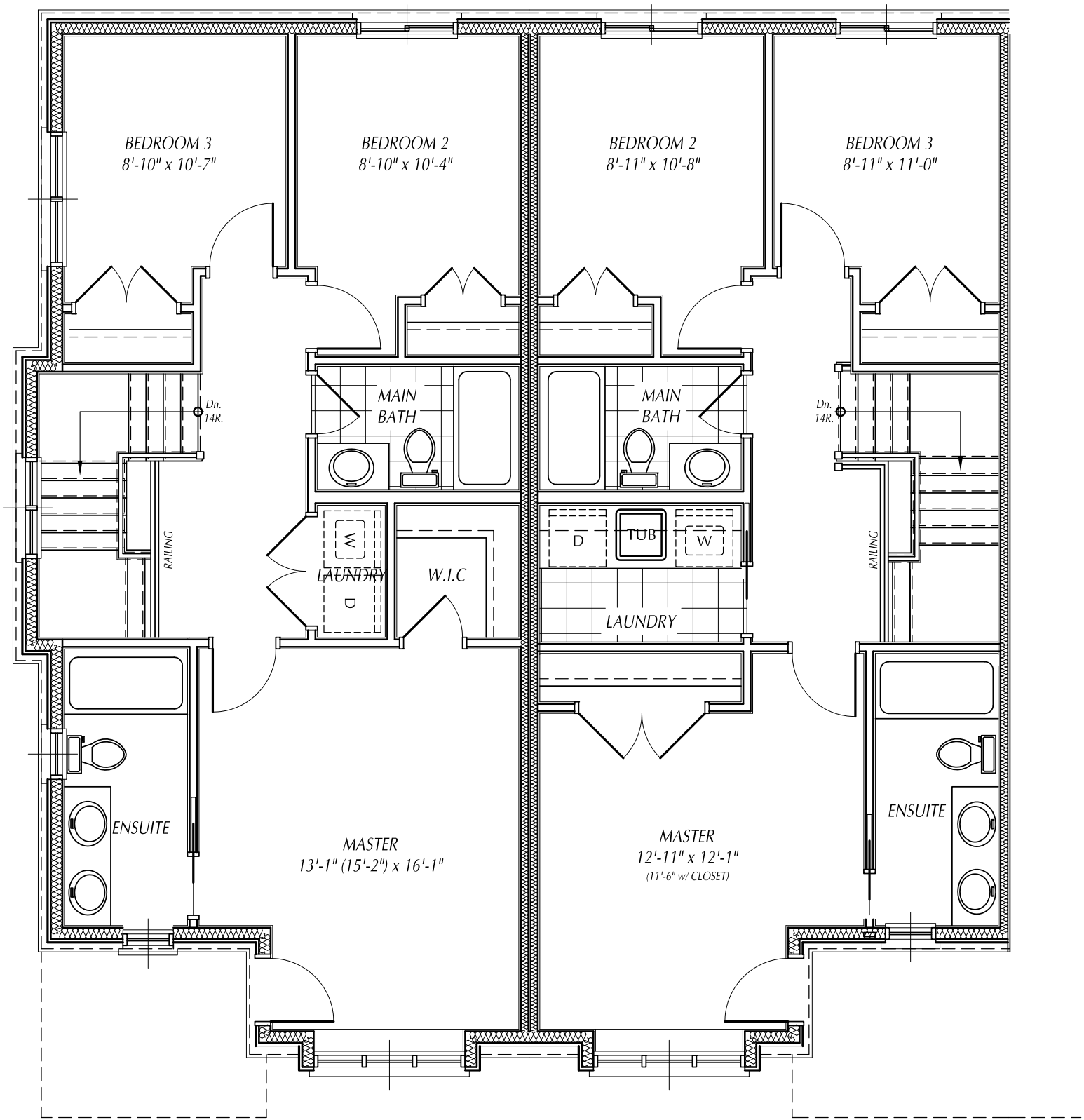
INTERIOR UNIT Second FLOOR PLAN Woolwich St.(Perks)
